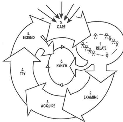
Abb. 1: CREATER-Modell von Havelock & Zlotolow (1995, 11)
